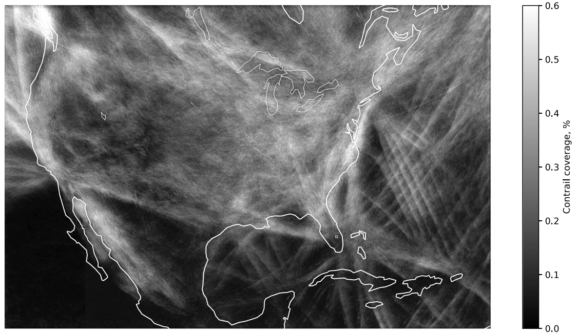
Figure 1. Mean contrail coverage from 1 January 2018 to 31 December 2019. Pixel intensity indicates the percentage of time during which a contrail was observed in that location. Each pixel is the average of approximately 70 000 individual observations. Some imperfections, such as scanline artifacts detected as contrails, are visible. These are removed before further analysis (see methods).
