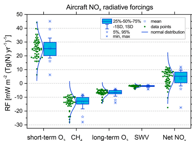
Fig. 4. Results from an ensemble of 18 models from 20 studies for aviation \text{NO}_x impacts: short-term \text{O}_3 increases; \text{CH}_4 reductions, \text{CH}_4 -induced long-term reductions of \text{O}_3 , \text{CH}_4 -induced reductions of stratospheric water vapor (SWV) and Net \text{NO}_x . Each data point represents a value of RF per unit emission ( \text{mW m}^{-2} (\text{Tg (N) yr}^{-1})^{-1} ) as normalized from a published study (see SD). \text{CH}_4 -induced \text{O}_3 and SWV are calculated using standardized methodology (see text for details). Note that the displayed values do not include correction factors to account for the non-steady-state \text{CH}_4 responses to \text{NO}_x emissions and the new \text{CH}_4 RF parameterization. These adjustments are applied in forming the best estimates as discussed in Appendix D.
